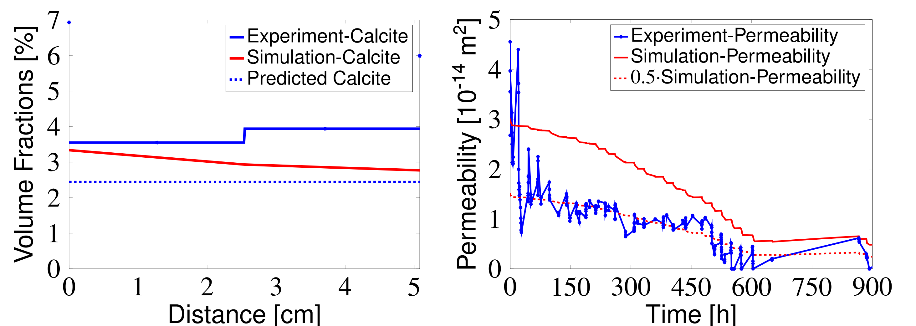
Figure 4: Comparison between experimental data and simulation results for MICP in a 2.54cm diameter sandstone core (see top picture in the middle of Figure 2) under reservoir pressure conditions. Measured and predicted volume fraction of calcite compared to simulation results after 21 MICP injection cycles (left). Permeability calculated from experimental pressure difference versus simulated permeability (right).
