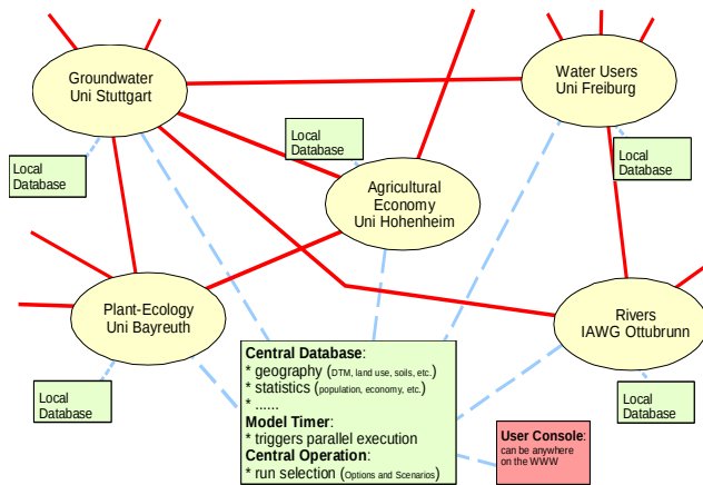
Fig. 4: Cut-Out of the Market Place Concept of Networking of the Participating Groups in the Project. Ellipses show groups, which exchange (offer and receive) dynamic data through solid lines and are supplied with static data from a Central Data Base
