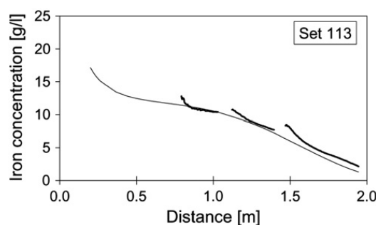
Fig. 9. Result of cascading column experiments using injection conditions specified in Materials and methods and a discretization of 7 columns of different length (thick lines) and mathematical model prediction according to Comba and Braun (2012) (thin line). Four columns reproducing the region near the well are excluded from the analysis due to their short length.
