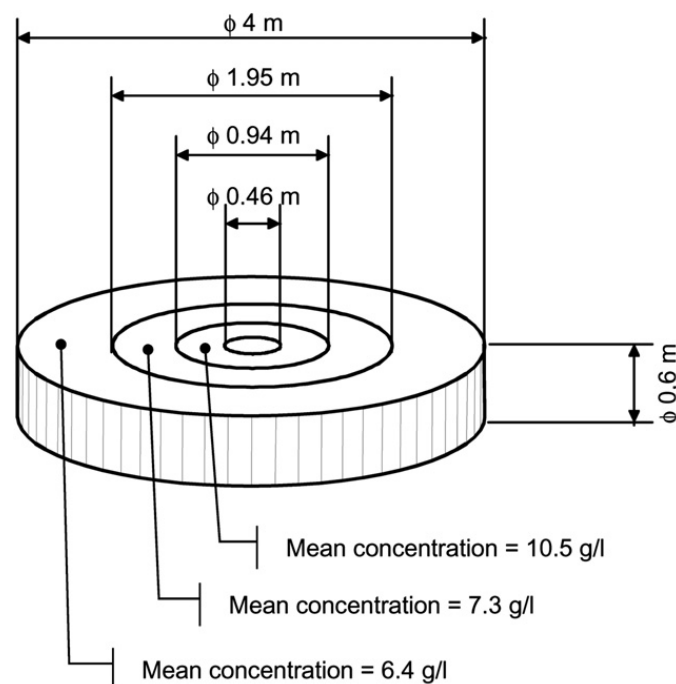
Fig. 4. Model cylindrical domain discretized into 3 shells following the criterion \bar{q}_{i+1}/\bar{q}_i = \text{const.} The results of the cascading column tests reported in Fig. 3 are reported for each shell in terms of average concentration of iron particles measured in each column.
